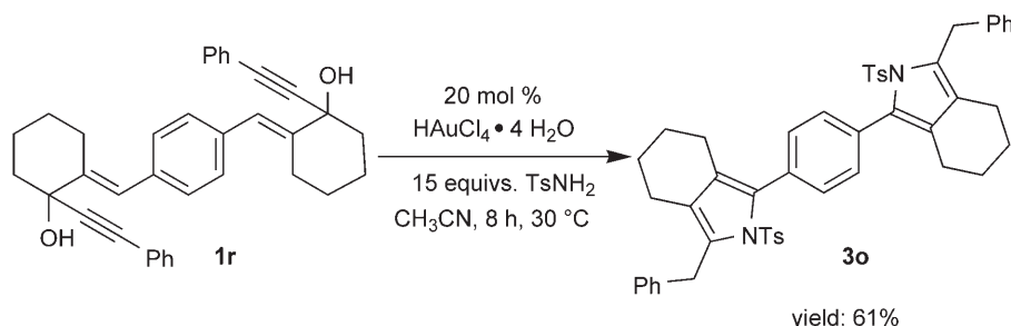
Scheme 2. One pot synthesis of bis(pyrrol-2-yl)arylene 3o .
