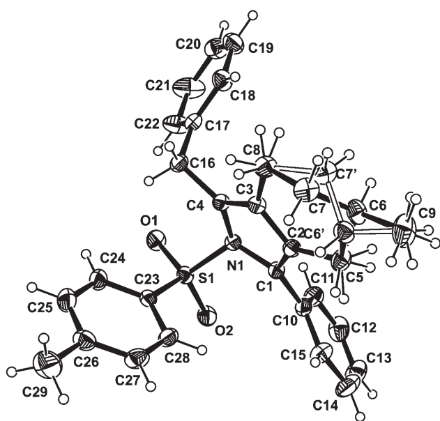
Figure 1. X-ray structure of 3n .
