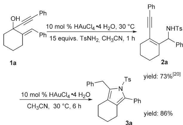
Scheme 3. Two-step synthesis of pyrrole 3a .
