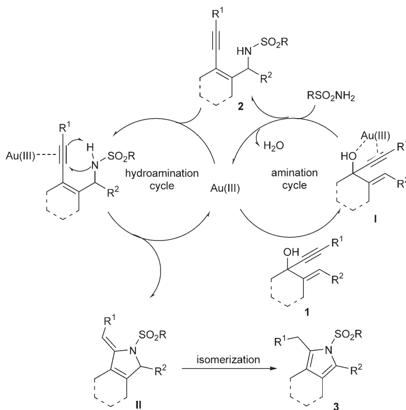
Scheme 1. Proposed gold(III)-catalyzed synthesis of substituted pyrroles.
